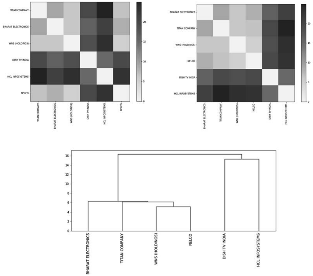
Fig. 6. Resultant heatmaps and dendrogram by Amplitude-based clustering method with computer manufacturers' data.
